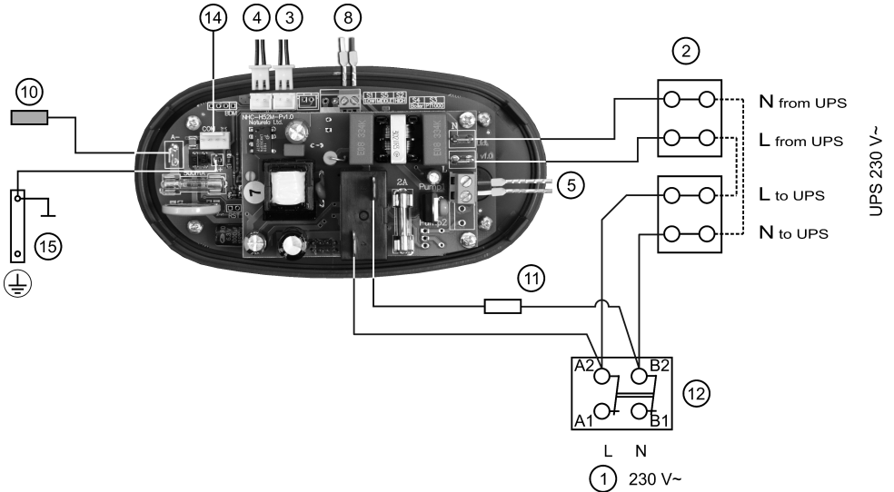
Fig. 1 Single-phase connection of water heaters with one heat exchanger NHC-H52M-1-1
