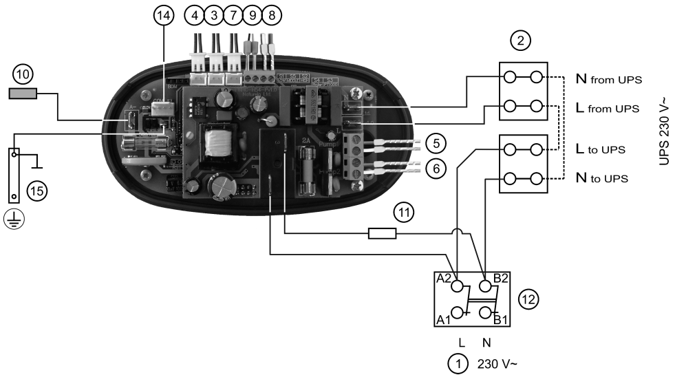
Fig. 2 Single-phase connection of water heaters with two heat exchangers NHC-H52M-2-1
