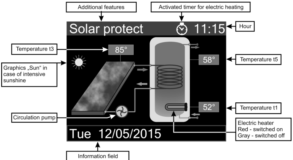
Fig. 3 - Display for electronic units NHC-H52M-1-1
