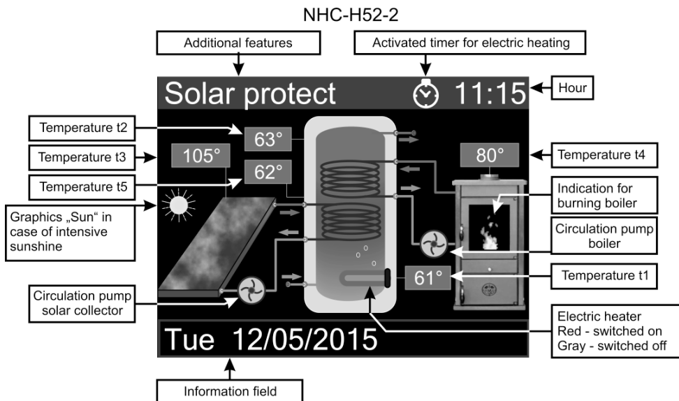
Fig. 4 - Display for electronic units NHC-H52M-2-1
